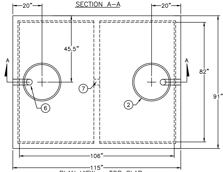
NOT TO SCALE PLAN VIEW - TOP SLAB
